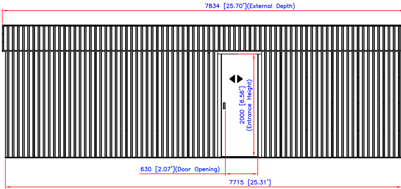
SIDE VIEW
